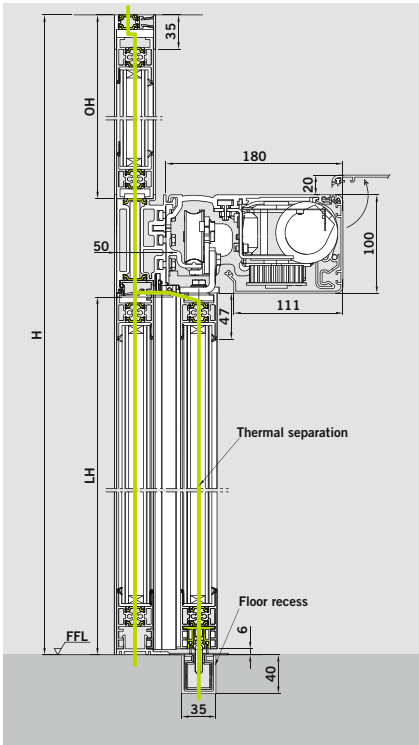
Corridor-mounted version with floor-integrated guide rail
