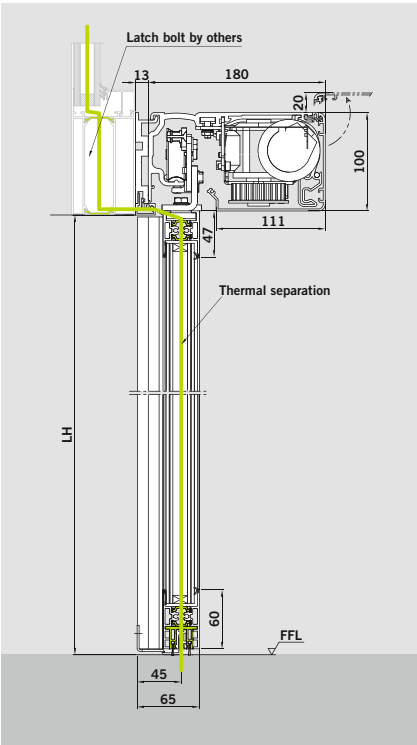
Lintel-mounted version installed on façade by others
