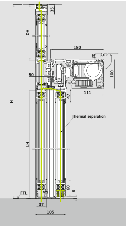
Corridor-mounted version with side screen and fanlight
