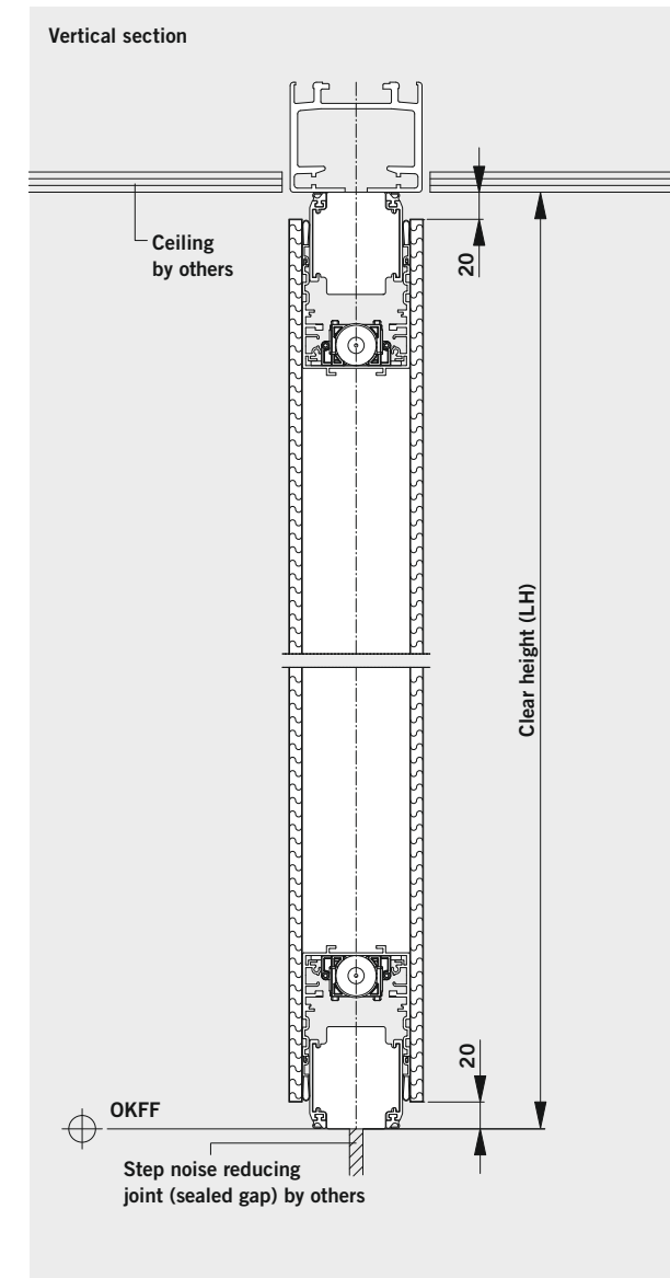
Visible edging (Type K)
