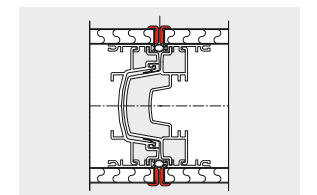
Protective casement edging (Type U)
